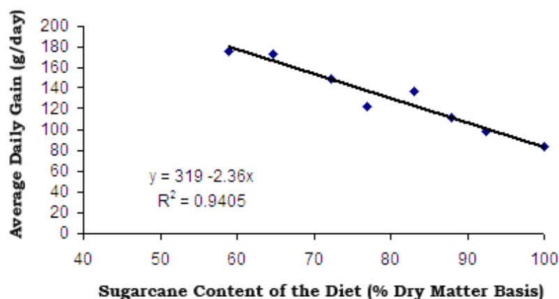
Figure 23: The relation between the quantity of sugarcane in the diet (% dry matter basis) and the average daily gain (g/day) of Martinique sheep. Source: Archimède (unpublished).
