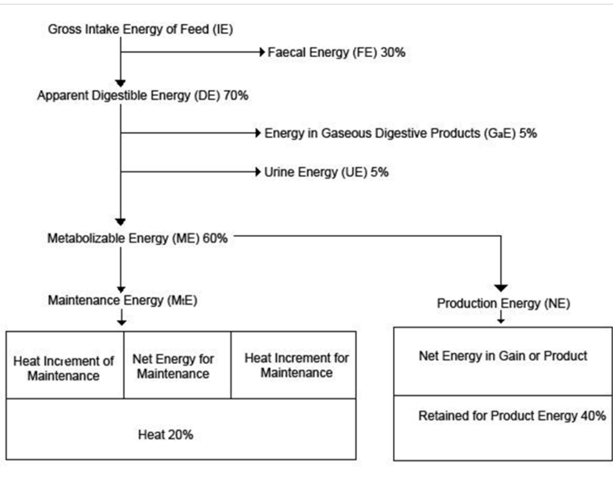
Figure 5a: A quantitative example of how the Gross Energy Intake of a ruminant is partitioned within the animal.
