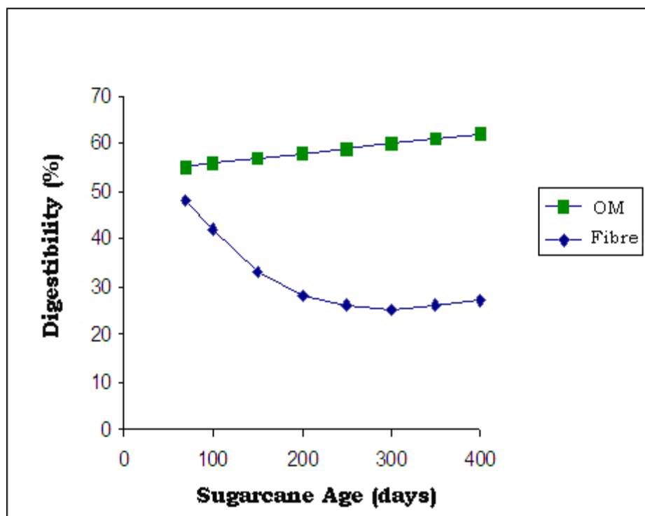
Figure 18: Changes in the organic matter [OM] and fibre digestibility of sugarcane (energy fractions) with age (Preston, 1976)
